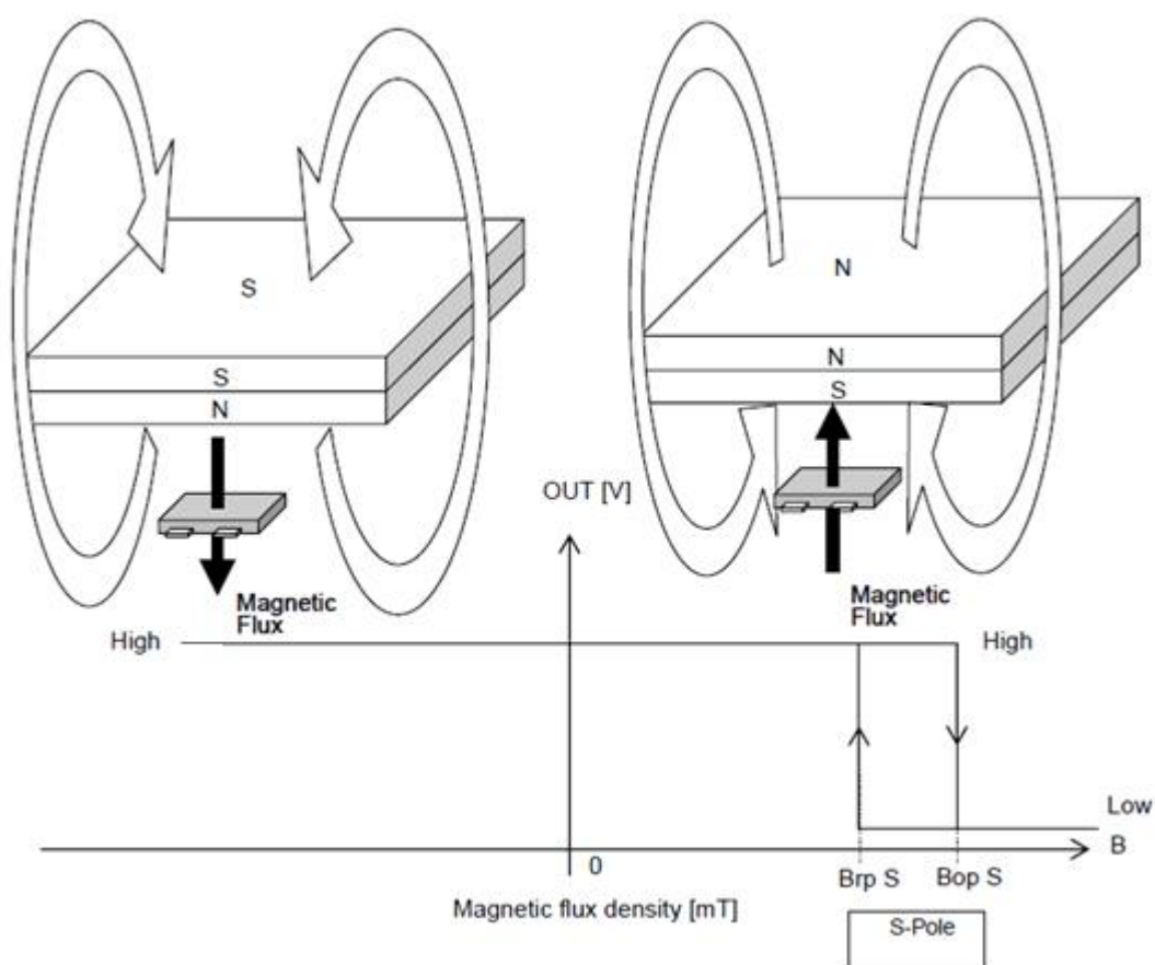
Fig 4, Magnetic Operation Characteristic of AS1510
