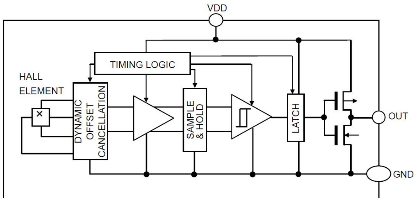
Figure 3, Block Diagram of AS1510
